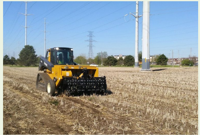
Figure 26: A front mounted seed drill on a skid steer spreading native seed in the spring.
